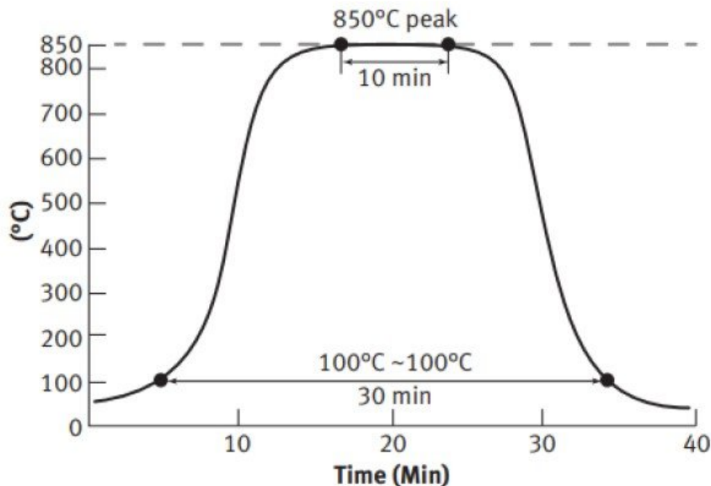
Micromax™ Standard QA Firing Profile (850°C 10 min)
